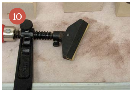
10 The Jaws 2 is another Fret Press. This one combines the fret caul with a big F clamp to give access to the upper fingerboard. Packing bits are included
