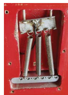
This old Strat trem has been set up as recommended by Carl Verhayan and the spring claw has ended up at an angle. It doesn't look pretty, but this Strat really stays in tune and the trem is very playable
