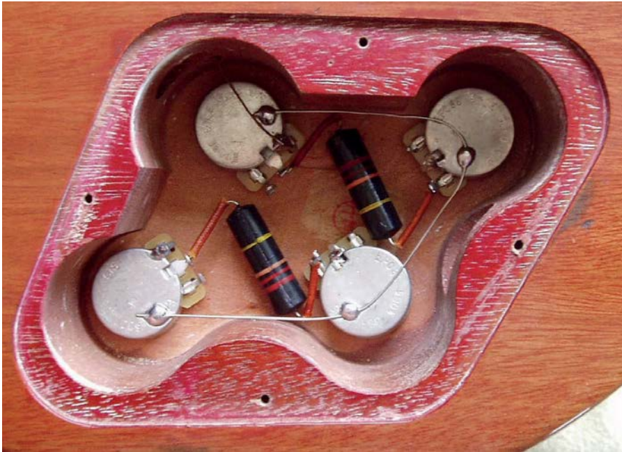
This picture shows the first stage of a '50s style wiring installation. Note how the 'bumblebee' capacitors are connected to the centre tags of the volume controls.
