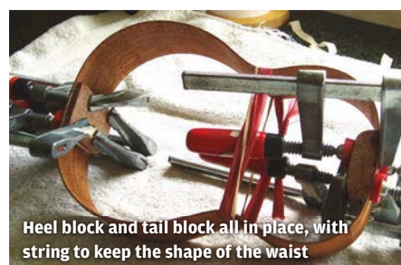
This jig keeps the shape of the body while you glue the box together
