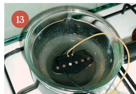
13 Potting the pickup Soaking the completed unit in wax helps prevent microphonic feedback
