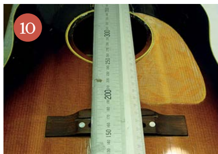
10 More checks making sure the neck lines up with bridge
