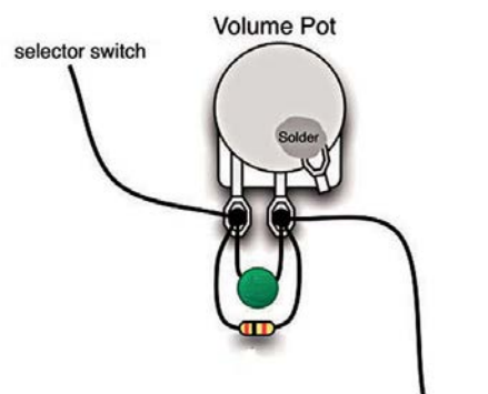
A treble bleed cap helps brightness when you turn down your volume. Some use a cap on its own; others prefer a resistor in series or – as shown here – in parallel with the cap.
