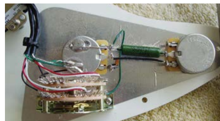
The pickup wires have been soldered to the switch as per the Seymour Duncan schematic. We prefer to keep cable runs as short as possible and the excess green wire we snipped off was used to connect the switch to the volume pot
