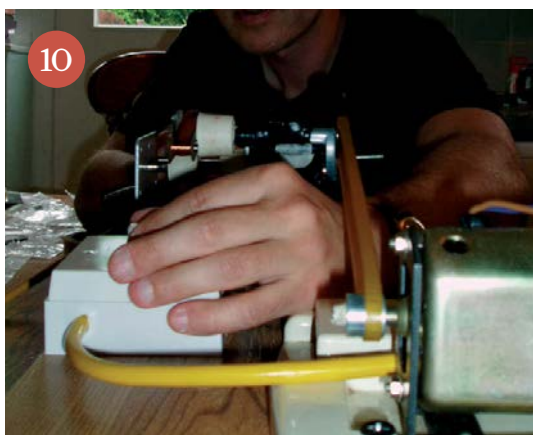
9 Tele-style pickup ready for baseplate gluing
