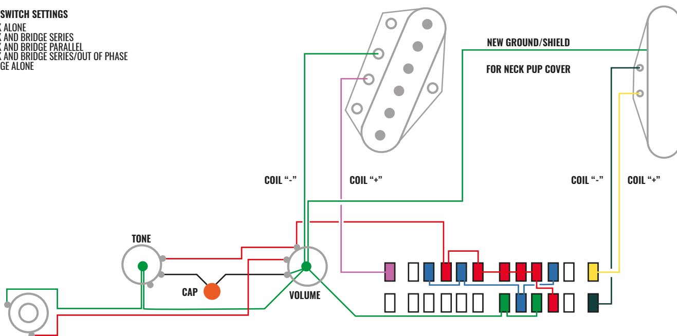
THIS IS TYPICAL WIRING FOR A TELE CONTROL PLATE, FLIPPED OVER AND SEEN FROM THE BOTTOM
